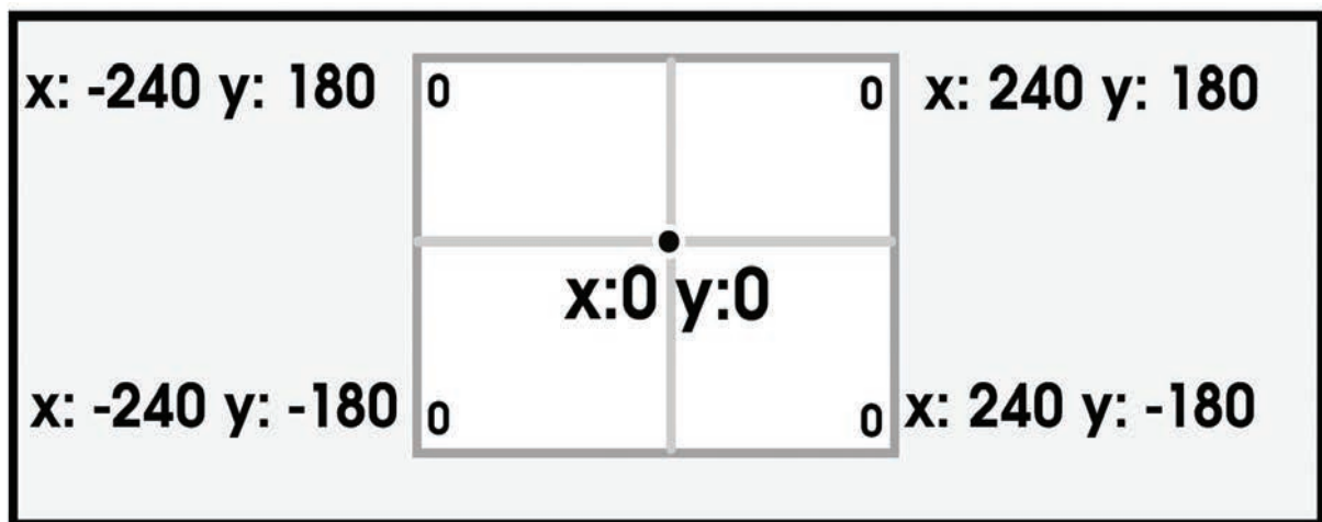
Fig. 8.8: Coordinates of X-Y plane (stage)
