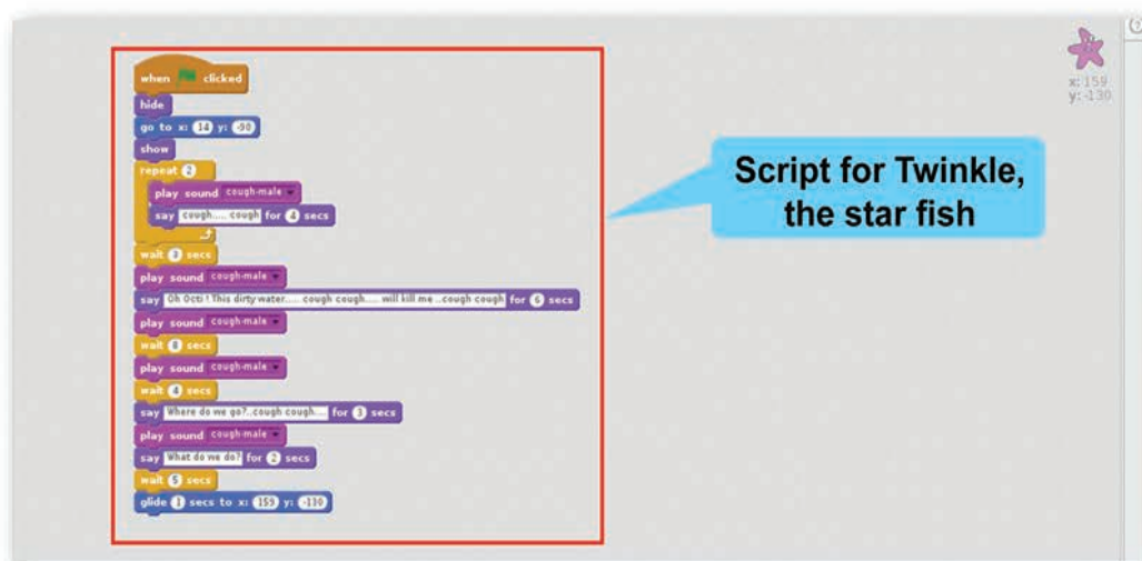
Fig. 8.13: Forming a script for Starfish Sprite
