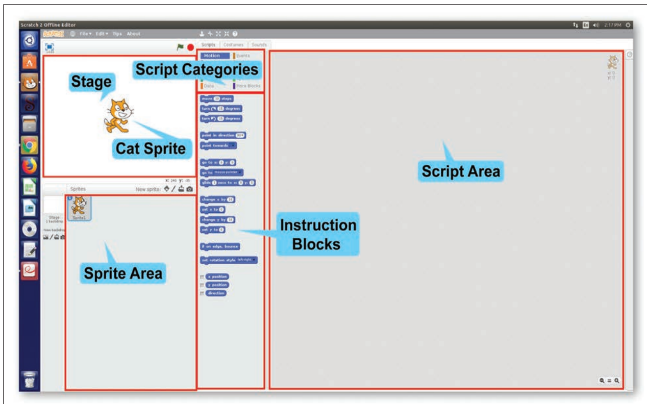
Fig. 8.3: Scratch Interface
