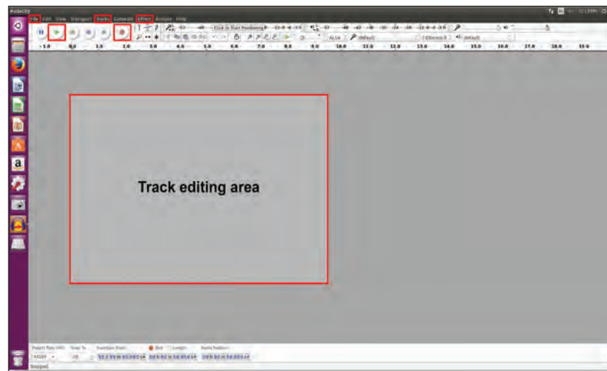
Fig. 4.1 : Audacity Interface
