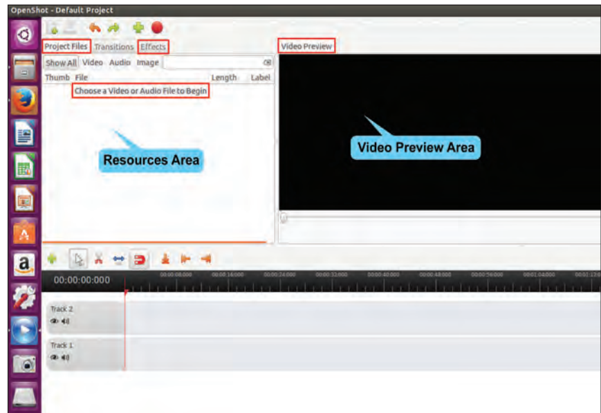
Fig. 4.8 Openshot Interface
