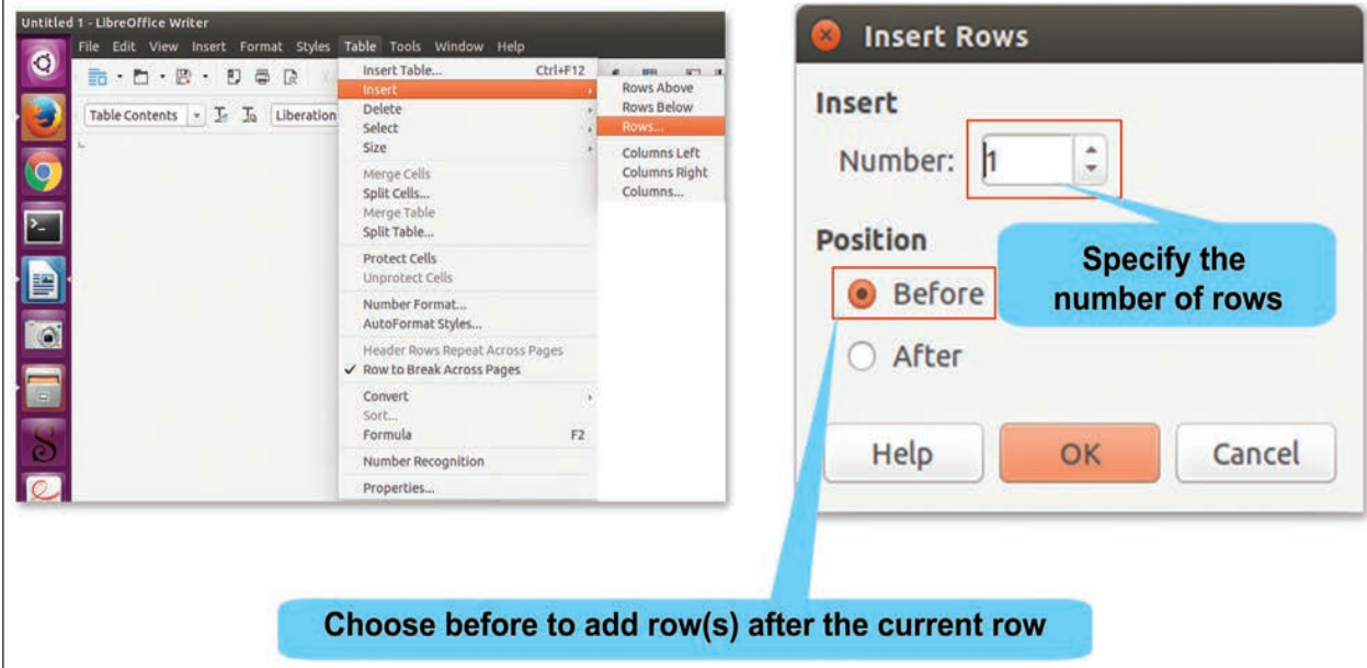
Fig 2.21: Inserting Rows in a Table
