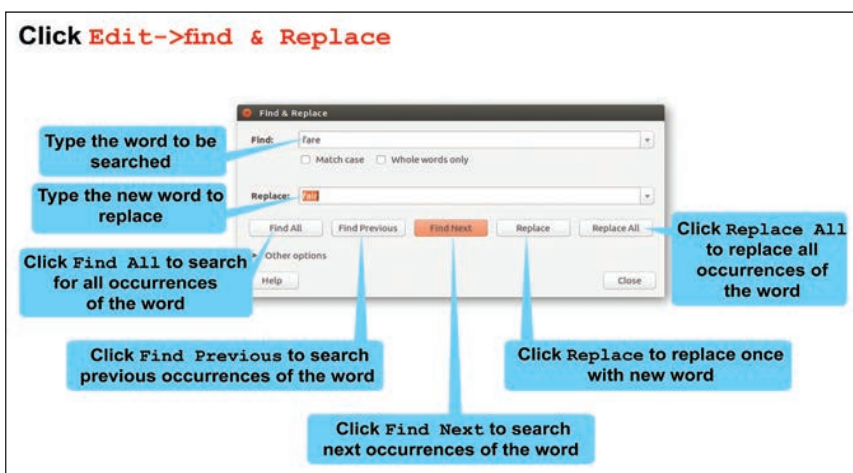
Fig. 2.16: Find and Replace
